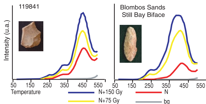
samples show a multicomponent signal, with the pTRM from the heating event being removed at ~350° and 450°C, respectively. (C) TL has not been zeroed on the untreated experimental sample (left) and is fully saturated (no increase of the signal with dose). The TL signal increased with the given dose on the heated experimental sample (right). (D) The archaeological samples resemble the unsaturated, heated experimental samples, because the TL signal still increases with the given dose.
